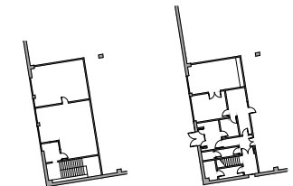
MEZZANINE FLOOR PLAN EXISTING 1:125
