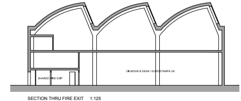
SECTION THRU FIRE EXIT 1:125
